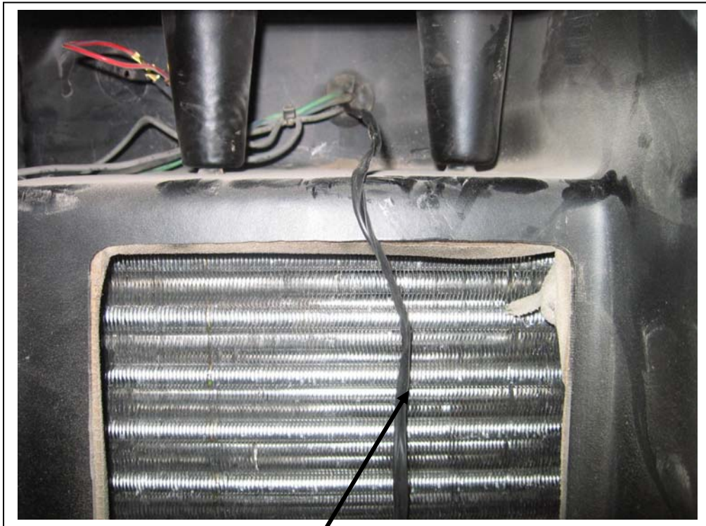
Thermostat probe.
